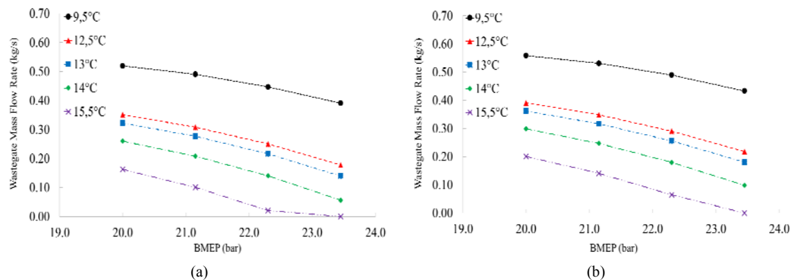
Figure 4. Wastegate mass flow rate versus brake mean effective pressure and air temperature with \Delta T_{CA} of (a) 8°C and (b) 2°C.
