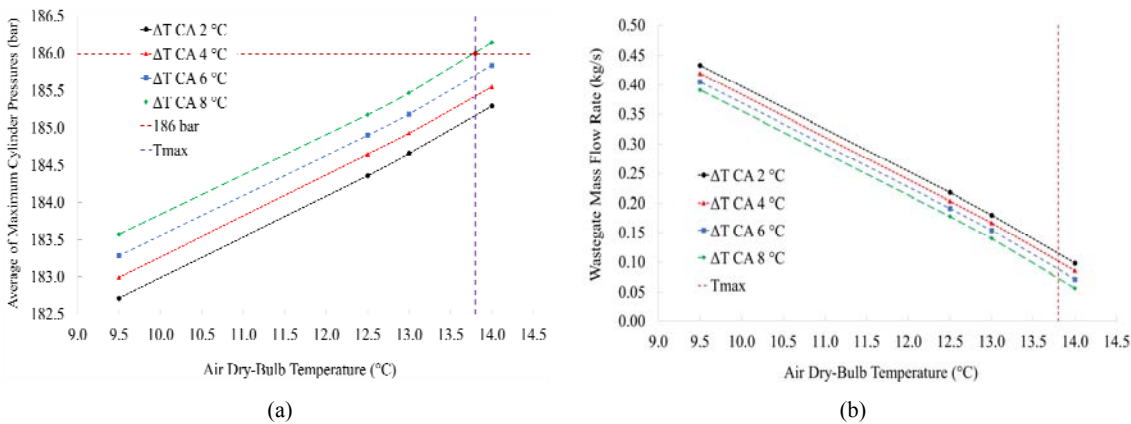
Figure 6. (a) Average of maximum cylinder pressures and (b) wastegate mass flow versus compressor inlet air temperature and \Delta T_{CA} with BMEP of 23.45 bar.
