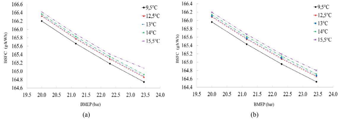
Figure 3. Brake specific fuel consumption versus brake mean effective pressure and air temperature with \Delta T_{CA} equal to (a) 8°C and (b) 2°C.
