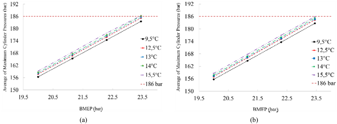
Figure 5. Average of maximum cylinder pressures versus brake mean effective pressure and air temperature with \Delta T_{CA} equal to (a) 8°C and (b) 2°C.
