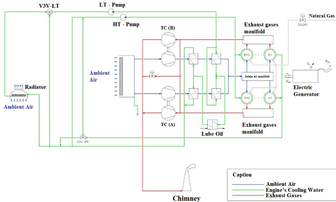
Figure 1. W20V34SG generator set flowsheet.
