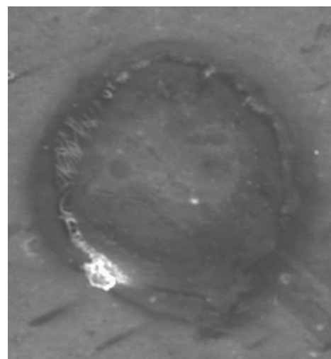
Figure 6. Aluminum after 5 hs in cavitating conditions. 100x, Pit 2.
