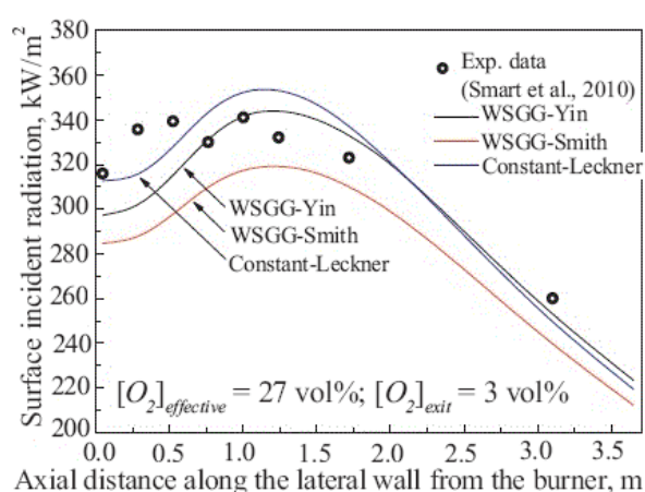
Figure 2. Surface incident radiation calculated with specific absorption coefficient model (Hu and Yan, 2013).
