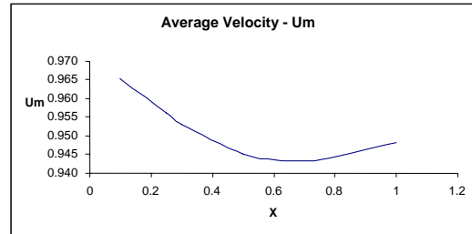
Figure 2. Average velocity of development along the axial position for Re = 20 and NU = NP = 50
