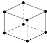
Figure 4. Element DC3D8 - 8 nodes and linear formulation (Hibbit et al. , 2007).
