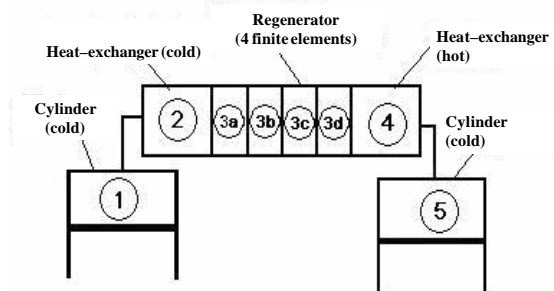
Figure 2. Division of the Stirling engine in different volumes or finite element to the PROSA software (Adapted from Thomas, 2003).
