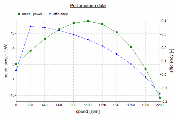
Figure 6. Influence of rotation on mechanical power and efficiency for the Amazon engine optimized by PROSA.
