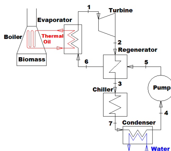
Figure 1. Organic Rankine cycle cogeneration.
