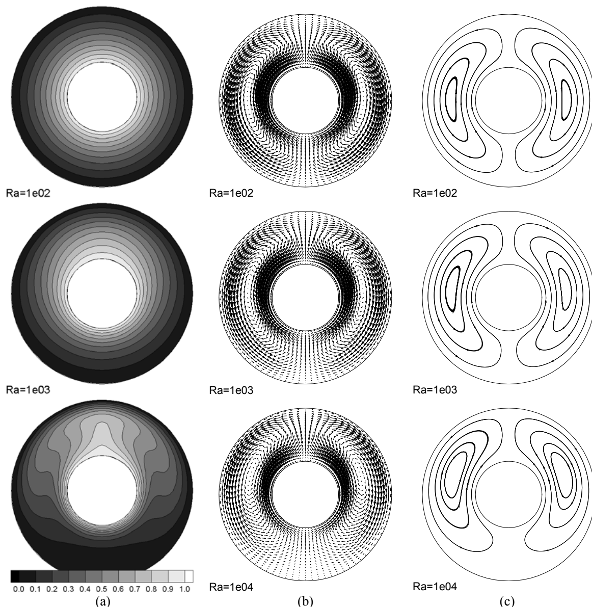
Figure 2. Isotherms (a), vector field (b) and streamlines (c) at three values of Ra , Pr = 0.71 , \eta = 2.6 , \Gamma = 1.0 .
