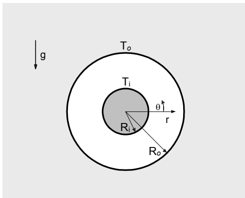
Figure 1. The two concentric cylinders configuration.
