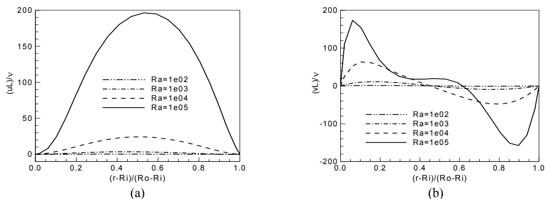
Figure 4. Velocity distribution at four values of Ra , Pr = 0.71 , \eta = 2.6 , \Gamma = 1.0 , radial velocity at \theta = 90^\circ (a), angular velocity at \theta = 0^\circ (b).
