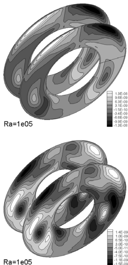
Figure 11. Isovalues of the axial velocity at Rayleigh number of 10^5 , Pr = 0.7 , \Gamma = 1.0 , \eta = 2.0 (up), \eta = 2.6 (down).
