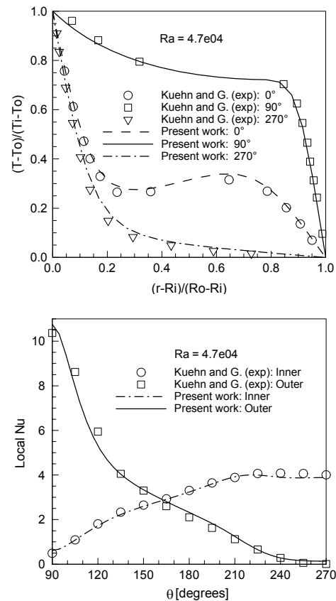
Figure 9. Comparison with experimental dates at Ra = 4.7 \times 10^4 , Pr = 0.71 , \eta = 2.6 , \Gamma = 1.0 , temperature distribution (up), local Nusselt number (down).
