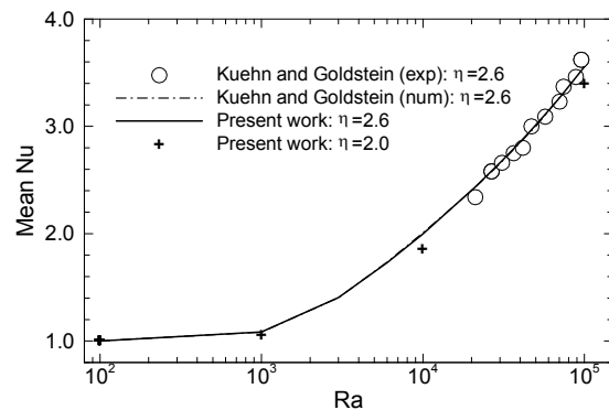
Figure 10. Comparison of mean Nusselt number with experimental and theoretical dates of Kuehn and Goldstein.
