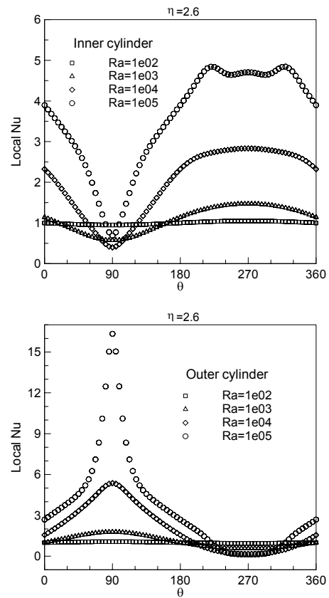
Figure 6. Local Nusselt number distribution at four values of Ra , Pr = 0.71 , \Gamma = 1.0 , inner cylinder (up), outer cylinder (down).
