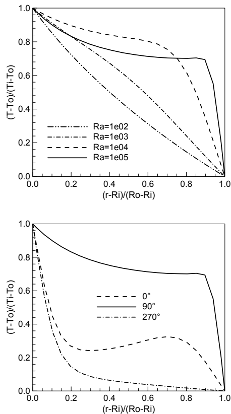
Figure 5. Temperature distribution, Pr = 0.71 , \eta = 2.6 , \Gamma = 1.0 , at four values of Ra and \theta = 90^\circ (up), at Ra = 10^5 and three values of the \theta (down).
