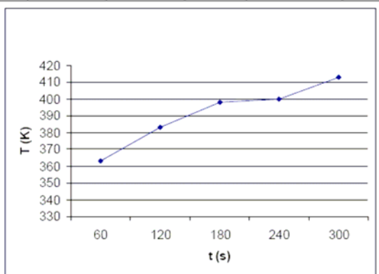
Figure 6. Variation of the temperature in the solar concentrator.
