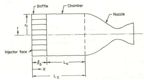
Figure 1. Combustion Chamber with a baffle.
