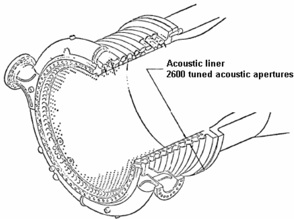
Figure 4. Position of acoustic liner along combustion chamber.
