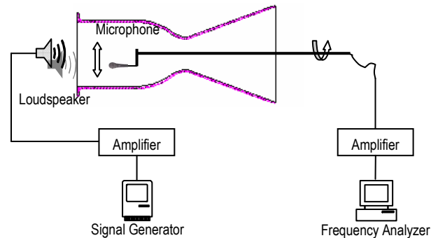
Figure 5. Experimental Setup.
