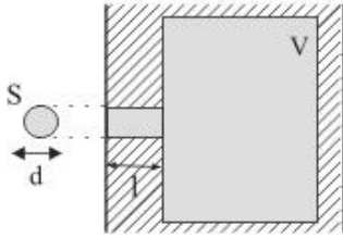
Figure 2. Helmholtz resonator.
