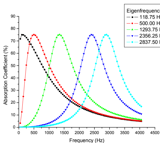
Figure 10. Absorption Coefficient for different eigenfrequencies.
