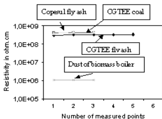
Figure 4. Comparison for different materials
