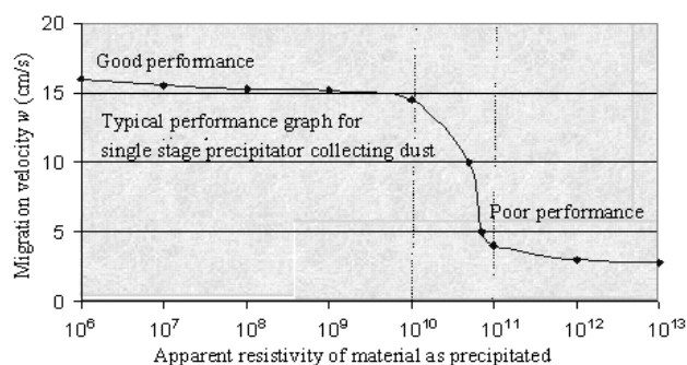
Figure 1. Effect of particle resistivity on ESP performance (White, 1962)
