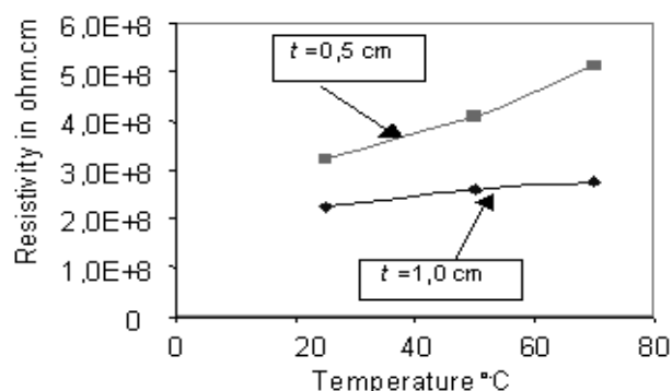
Figure 3. Influence of temperatura on resistivity
