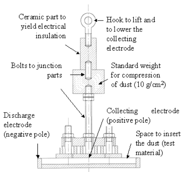
Figure 2. Description of experimental apparatus
