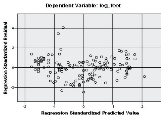
Scatterplot
