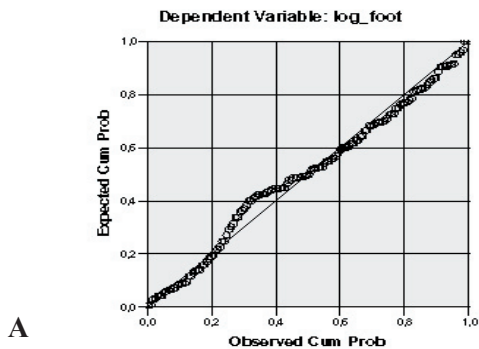
Scatterplot
