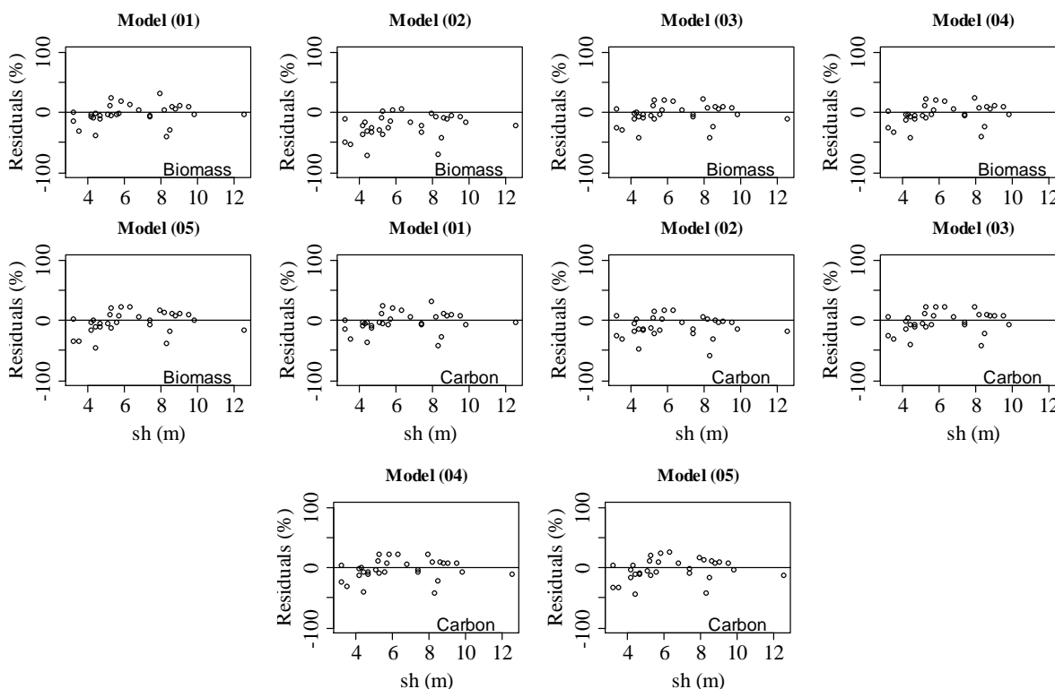
Figure 1. Residual dispersion of the tested models to estimate the biomass and above-ground total carbon of the Elaeis guineensis species as a function of the height of the stipe ( sh ).
