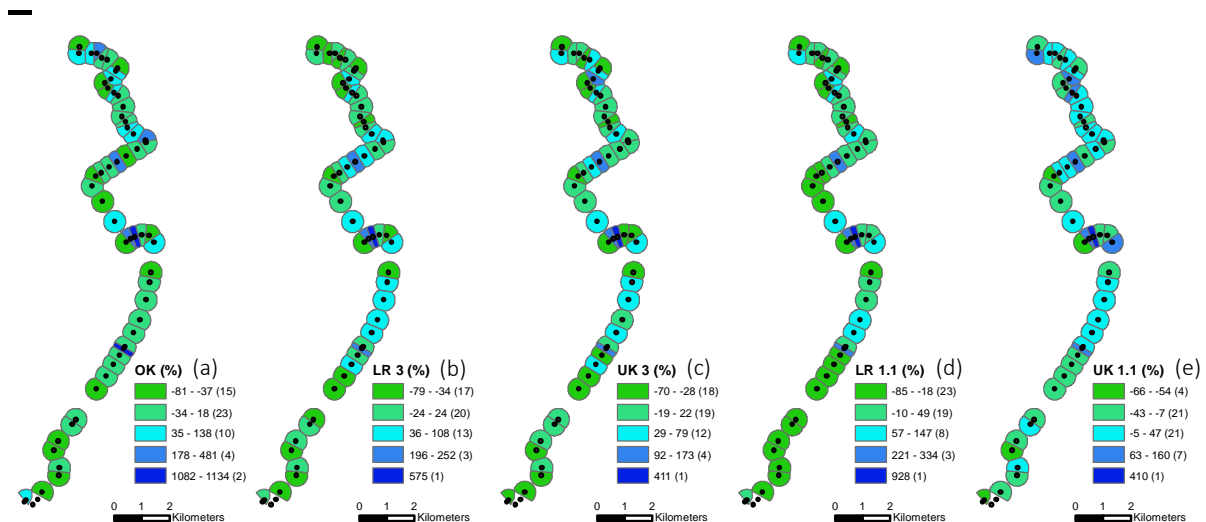
Figure 3: Error ratios of (from left to right) Ordinary Kriging (a), Linear Regression and Universal Kriging with all three predictors (b and c), and Linear Regression and Universal Kriging with ln_pop (d and e).
