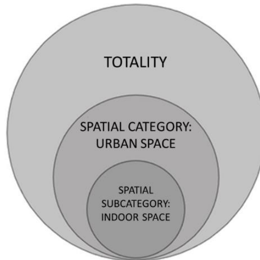
Figure 1: Spatial categories.
