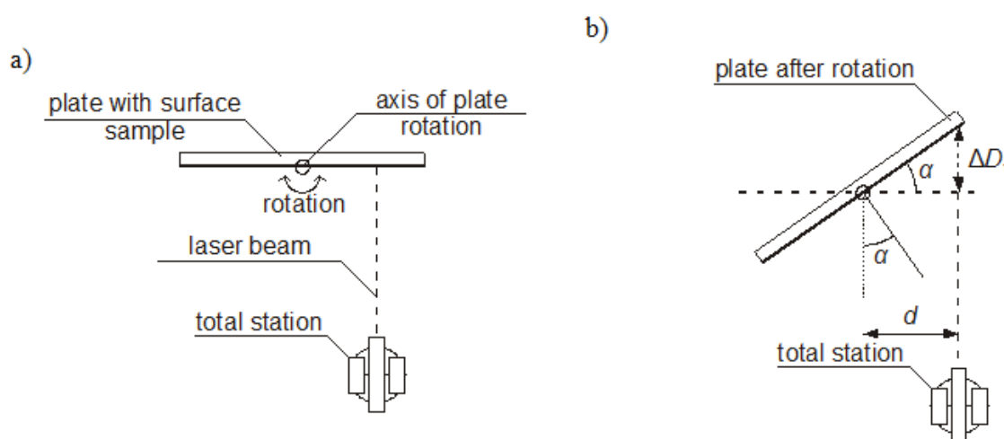
Figure 4: Scheme of systematic error source associated with the lack of intersection of the rotation axis and the direction of the laser light beam (a) and a scheme to calculate distance changes \Delta D_1 (b)
