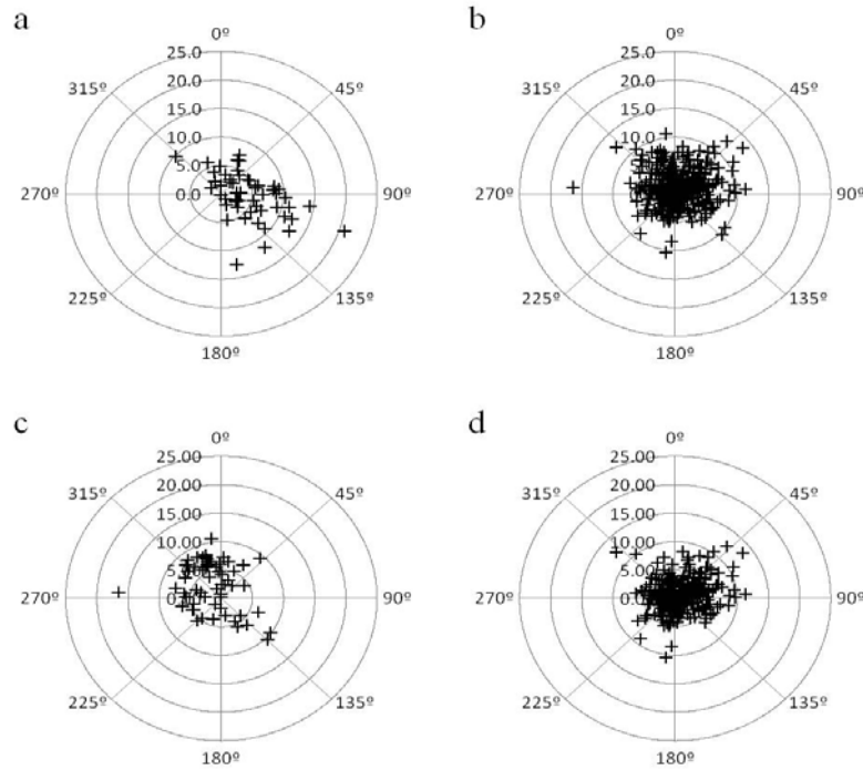
Figure 5 – GE's imagery horizontal error vectors for (a) 52 SPOT, (b) 414 DG, (c) 60 DG pre 2008 and (d) 354 DG post 2008 check points. Units: meters. North: 0°.
