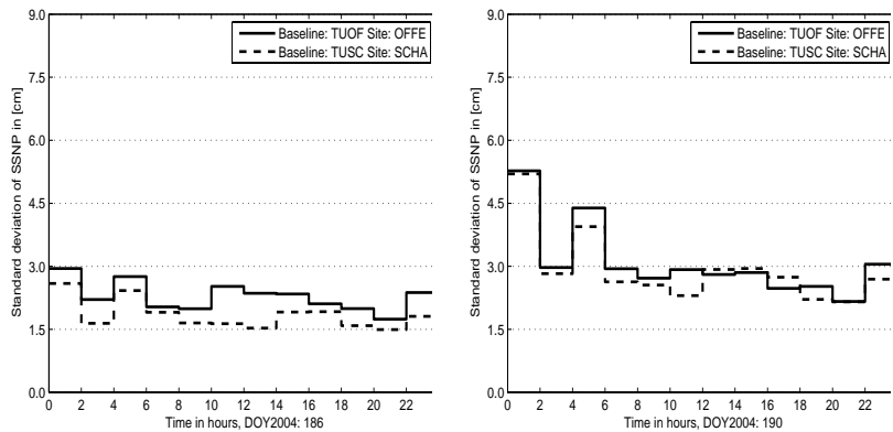
Fig. 5 - Comparison of the standard deviations of the SSNP concerning multipath and weather situation; left: DOY2004: 186, right: DOY2004: 190.
