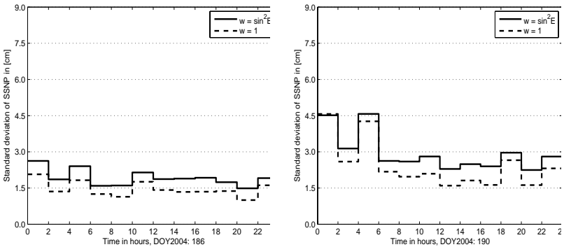
Fig. 6 - Comparison of the standard deviations of the SSNP concerning observation weighting and weather situation; left: DOY2004: 186, right: DOY2004: 190.
