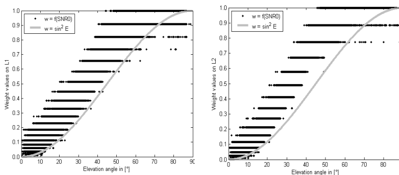
Fig. 8 - Comparison of the weight values of L1 and L2 observations (SNR-based vs. elevation-dependent), HLBR (Leica SR 520, LEIAT503), DOY2004: 186; left: weight values on L1, right: weight values on L2.
