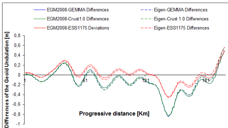
Figure 5: Differences between residual geoid heights computed with the global geopotential models EGM2008 and EIGEN-6C4 and the isostatic geoid height anomalies with GEMMA, CRUST 1.0 and ESS1175 crustal parameters.
